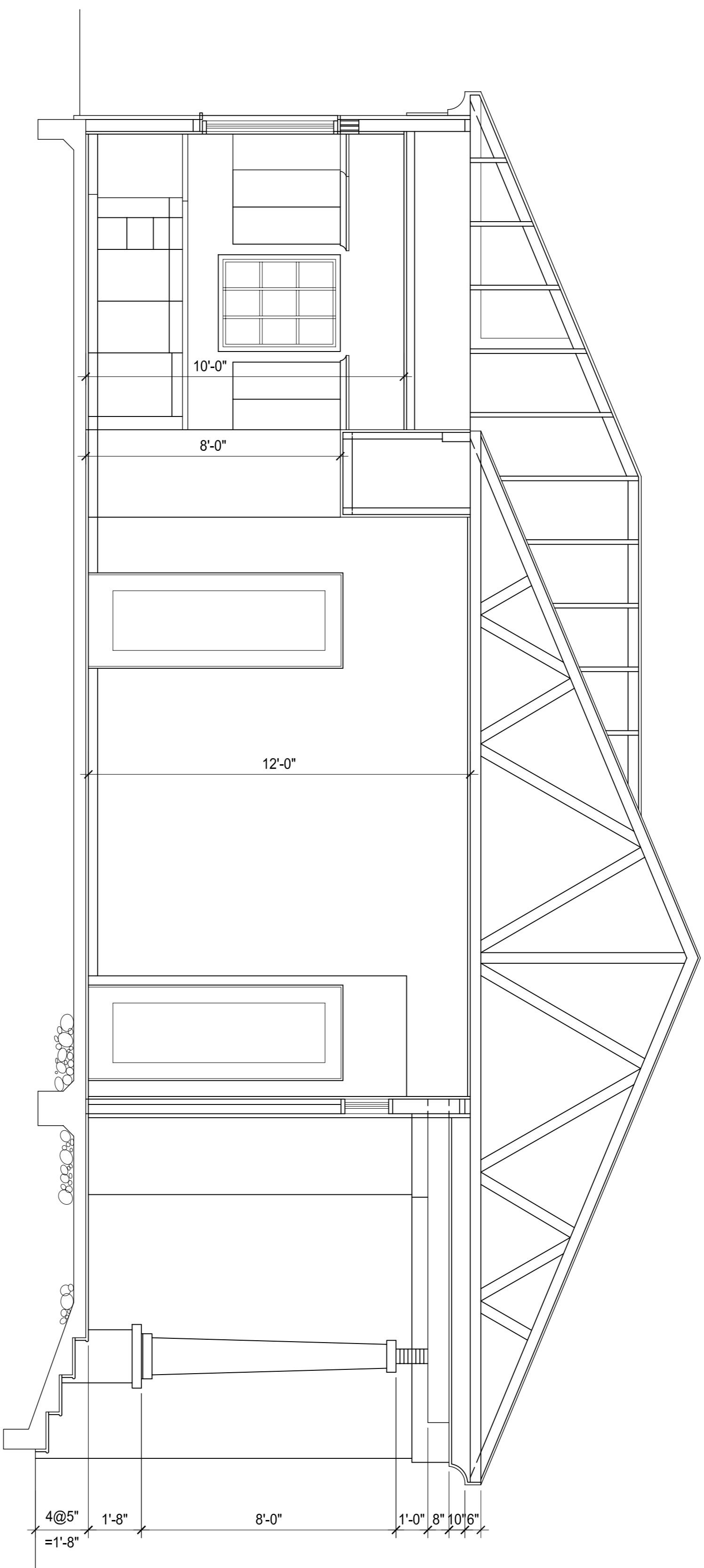
○ BUILDING SECTION SCALE: 3/8" = 1'-0"
