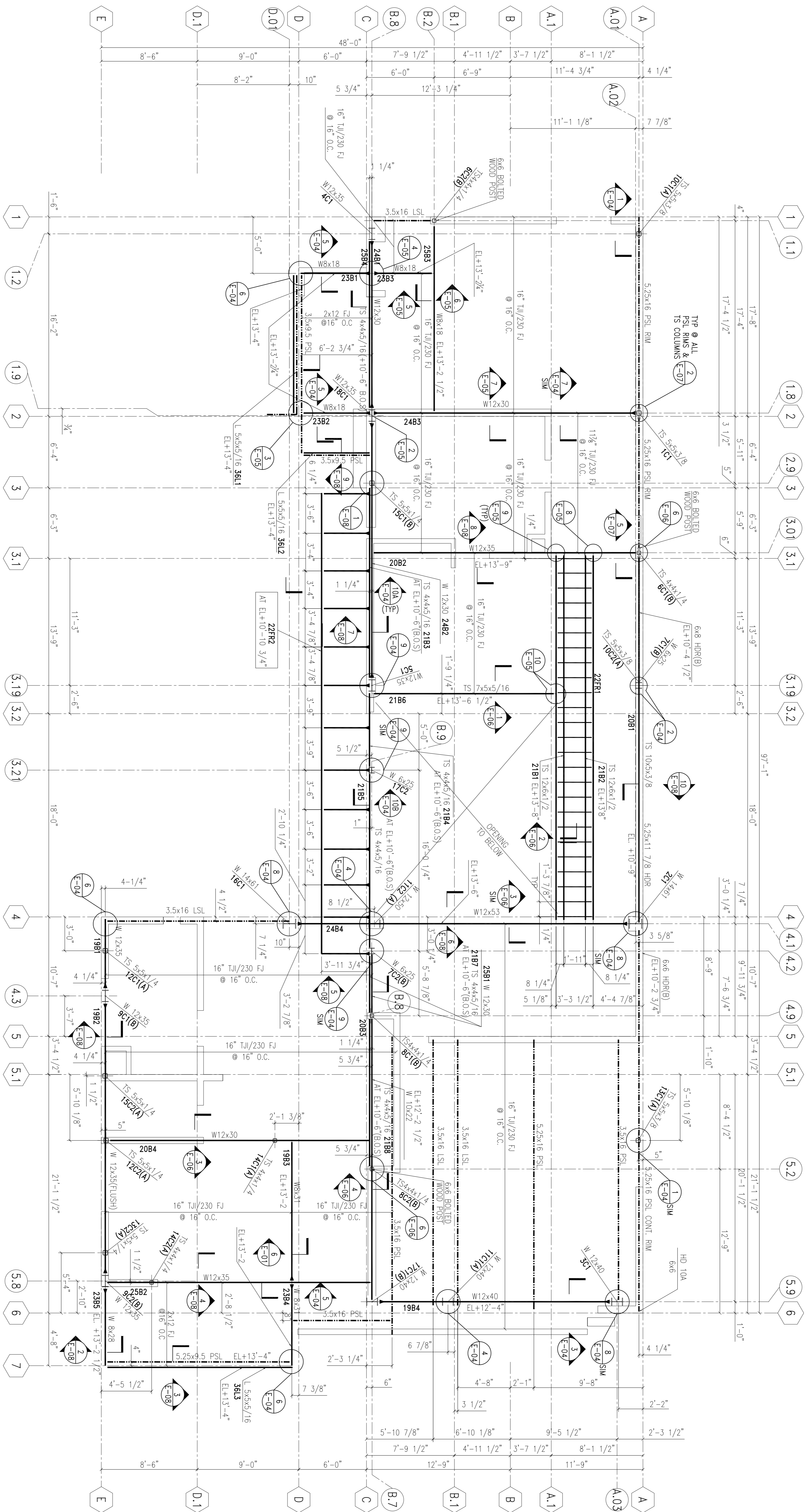
NORTH SECOND FLOOR FRAMING PLAN (T.O.S. EL. +13'-6 1/2" U.N.O.) (TOP OF WOOD BEAM EL. +13'-9 1/4" U.N.O.)
